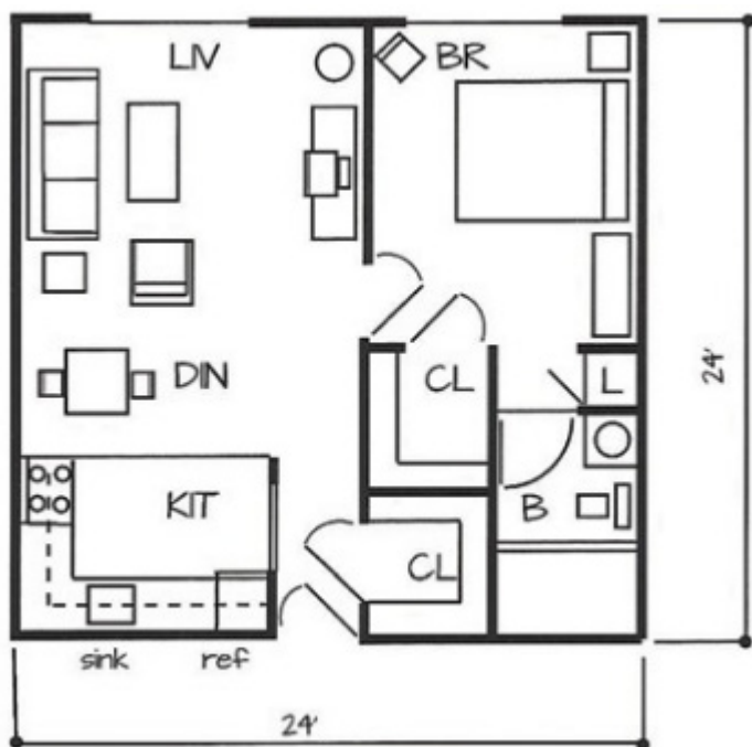
One Bedroom with Full Kitchen 576 sq. ft.
